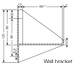
Wall bracket
