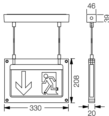
Surface ceiling mounting with Seilabhängung
