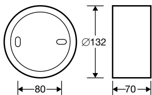
Ceiling tube
